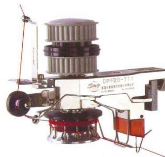
Product Name: CPF20-T11 YARN FEEDER (12V 24V) MAGNETIC YARN BREAKER Product Code: 01679 Introduction: CPF20-T11 YARN FEEDER (12V 24V) MAGNETIC YARN BREAKER
